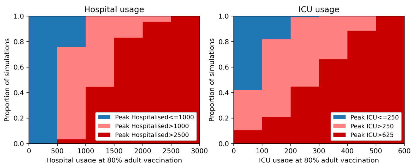
Figure 7: 80% two-dose vaccine coverage among people 16+ years time point. Estimated peak hospital and ICU demand, based on hospital and ICU demand at 80% two dose coverage. Left: proportion of simulations resulting in peak hospital demand <1000 (blue), 1000-2500 (salmon) or >2500 (red) for an observed hospital demand at the 80% coverage time point. Right: proportion of simulations resulting in peak ICU demand <250 (blue), 250-625 (salmon) or >625 (red) for an observed ICU demand at 80% coverage.
