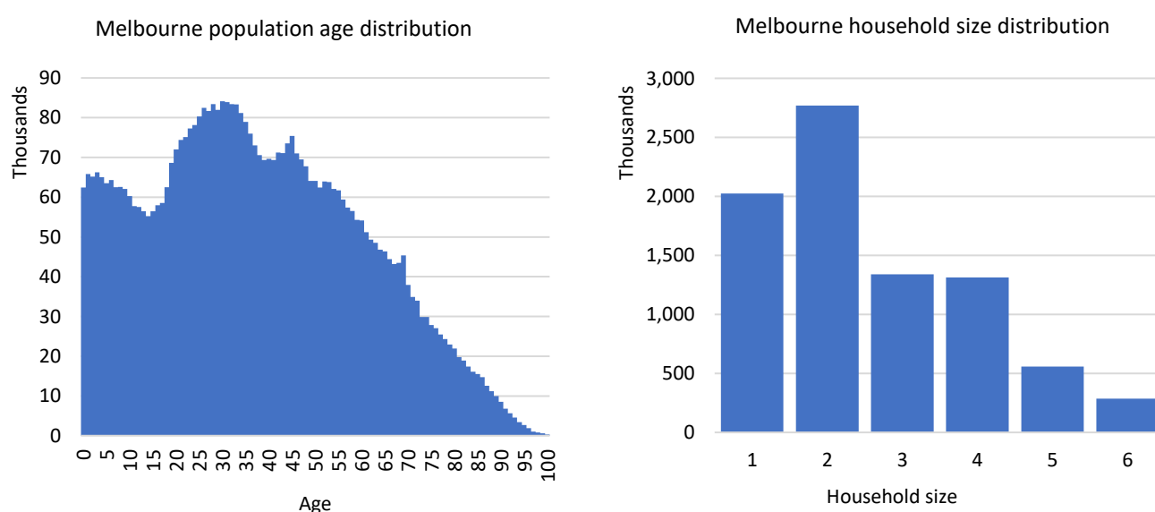
Figure S1: Population age structure and household size distribution [10].
