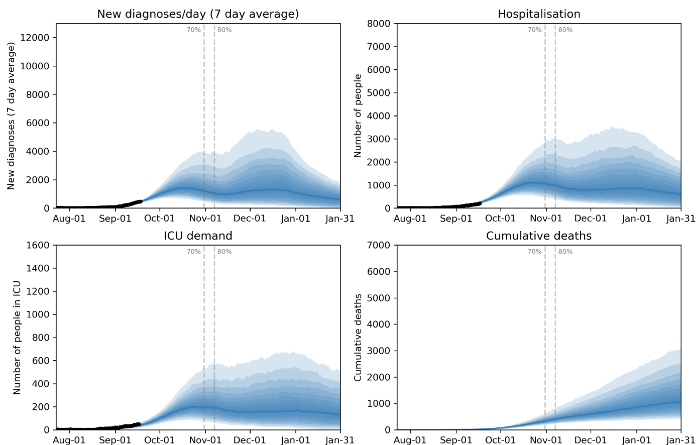
Figure 6: Roadmap scenario with a 15% reduction in non-household transmission. Eased restrictions based on Table 2 and Table 3 and mandatory vaccines; and in addition, an assumed 15% reduction in non-household transmission is implemented and sustained . It is unclear how this could be achieved, but would likely be a combination of targeted public health measures. This scenario illustrates that actions taken now can provide benefits later. Dashed vertical lines represent estimated dates of reaching 70% and 80% two-dose coverage among people 16+ years.
