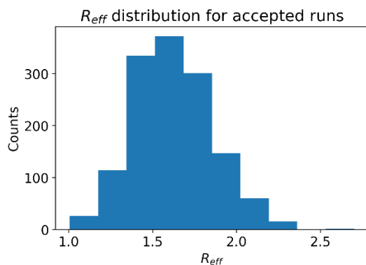
Figure S3: Accepted values for R_{eff} .
