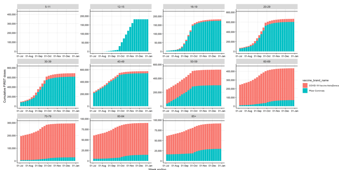
Figure 2: Cumulative FIRST dose coverage, used for model inputs. Second dose coverage is based on actual and proposed future changes to dose scheduling, and makes an approximation that everyone receiving a first dose receives a second dose. Red: AstraZeneca. Green: Pfizer.
