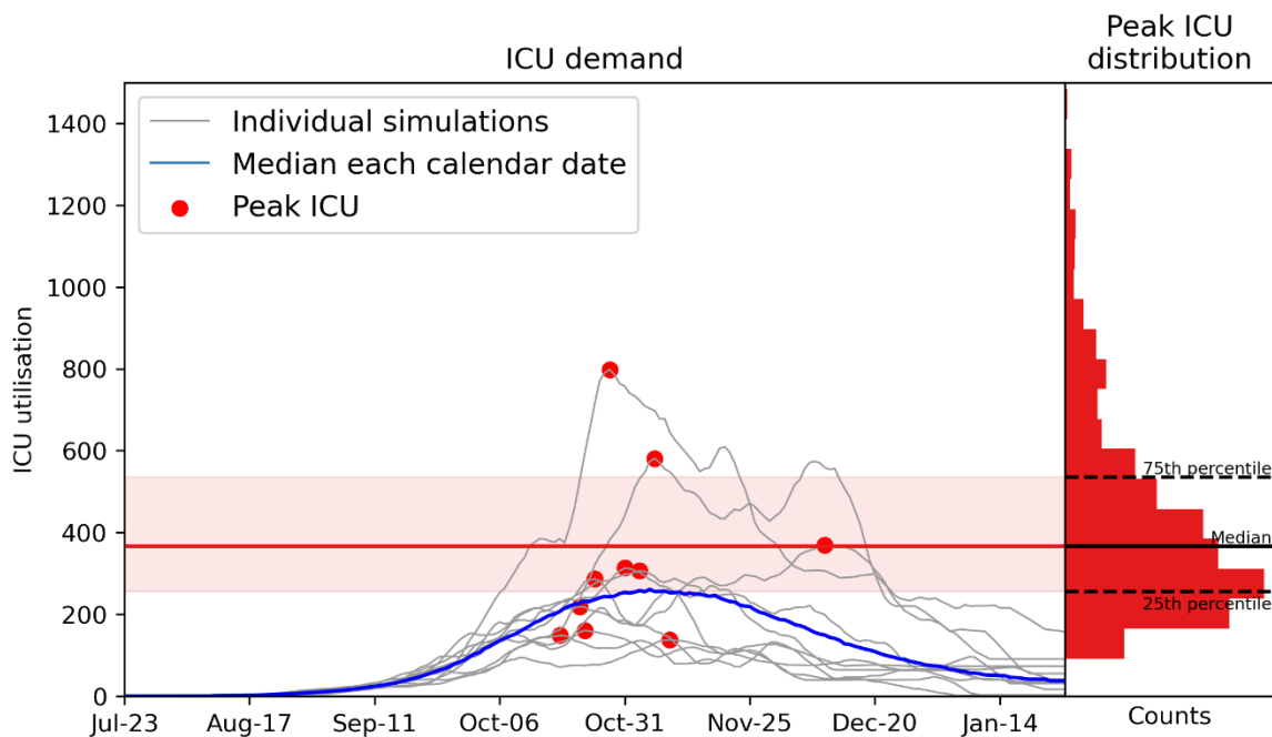
Figure S4: Median line over time, versus peaks of individual simulations.
