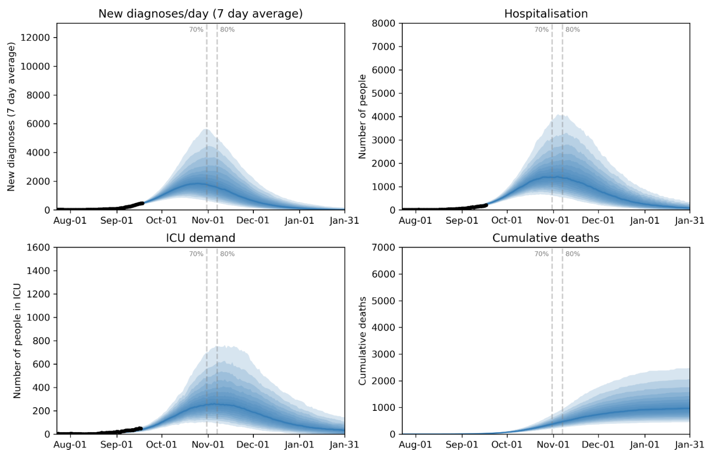
Figure 3: Maintain lockdown scenario. Figures show a counterfactual scenario where the lockdown is maintained, to provide a baseline estimate for easing of restrictions. Projected 7-day average daily diagnoses (top), hospital utilization (top-right), ICU utilization (bottom-left), and cumulative deaths (bottom-right). Dashed vertical lines represent estimated dates of reaching 70% and 80% two-dose coverage among people 16+ years.
