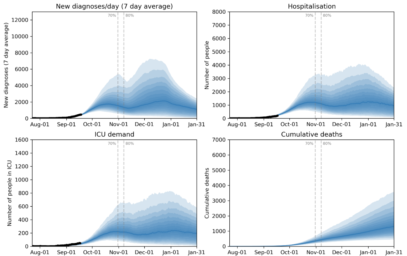
Figure 5: Roadmap scenario with increased testing. Eased restrictions based on Table 2 and Table 3 and mandatory vaccines; and in addition , vaccinated people are assumed to be equally as likely to seek symptomatic testing as much as unvaccinated people, even for mild symptoms. Dashed vertical lines represent estimated dates of reaching 70% and 80% two-dose coverage among people 16+ years.
