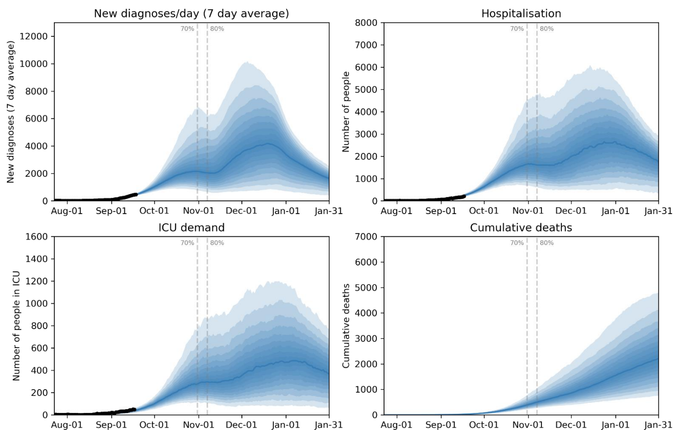
Figure 4: Roadmap scenario. Includes schools returning to in person learning throughout October; childcare returning and mobility restrictions easing in October; limited outdoor gatherings at 70% two-dose vaccine coverage among people 16+ years; indoor gathering with density limits at 80% two-dose coverage among people 16+ years (Table 2 and Table 3); and mandatory vaccine requirements. Dashed vertical lines represent estimated dates of reaching 70% and 80% two-dose coverage among people 16+ years.
