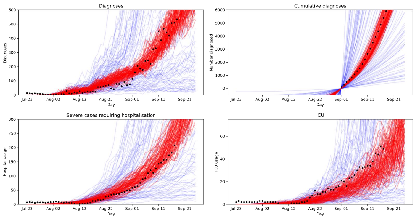
Figure S2: Model calibration to data from July-September 2021. Red lines indicate simulation runs that were maintained and used for this study; blue lines show a representative sample of simulations that were rejected. Cumulative diagnoses have been offset to prioritize calibration to most recent data.
