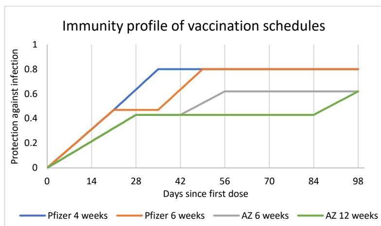
Figure 1: Vaccination immunity profile over time. Vaccinations were modelled according to vaccine type and time between doses and had a time-varying protection that depended on the vaccine type and time between doses.
